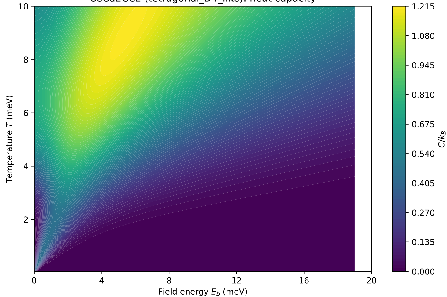
CeCu 2 Ge 2 (tetragonal_D4_like): heat capacity
