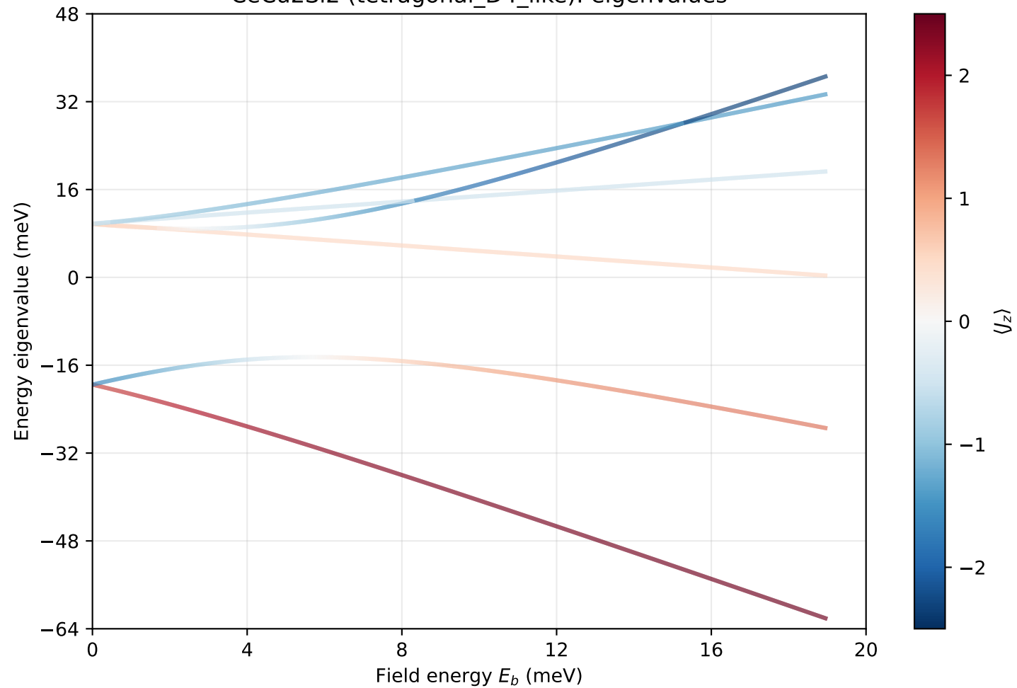
CeCu 2 Si 2 (tetragonal_D4_like): eigenvalues
