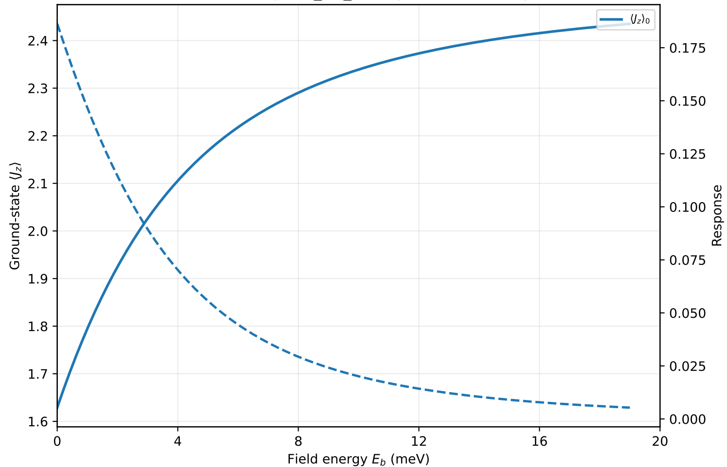
CeCu 2 Si 2 (tetragonal_D4_like): ground-state response
