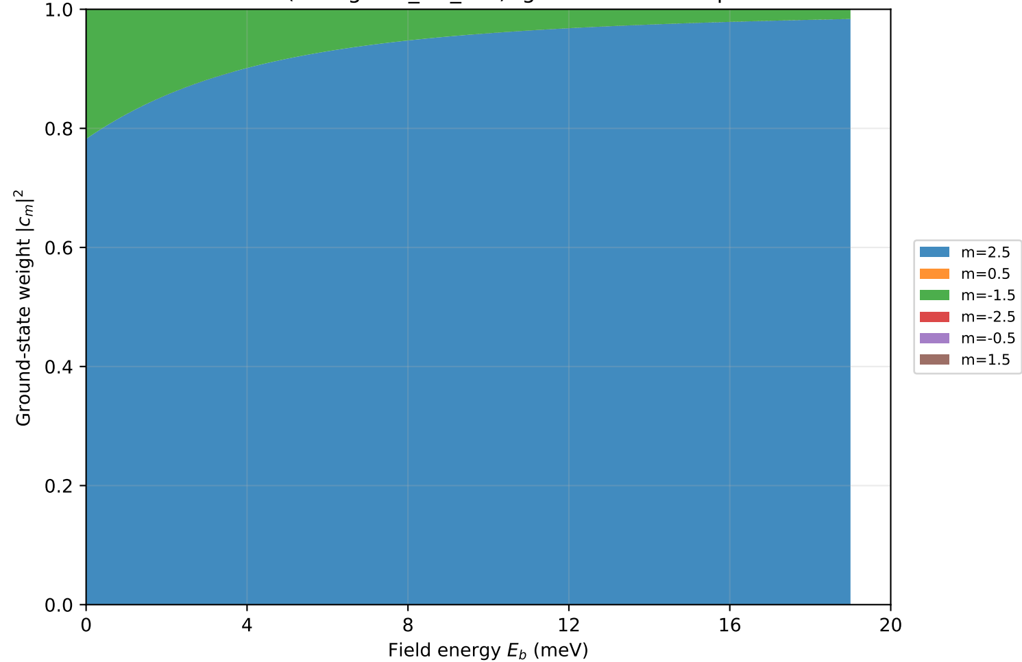
CeCu 2 Si 2 (tetragonal_D4_like): ground-state composition
