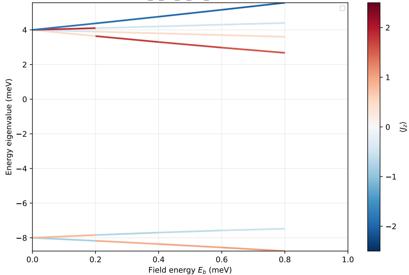
CeIn3 (cubic_B_Td_O_Oh_like): eigenvalues
