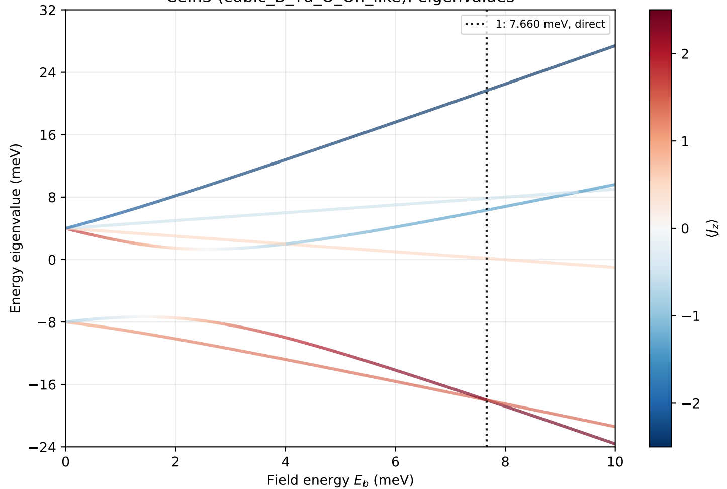
CelN3 (cubic_B_Td_O_Oh_like): eigenvalues
