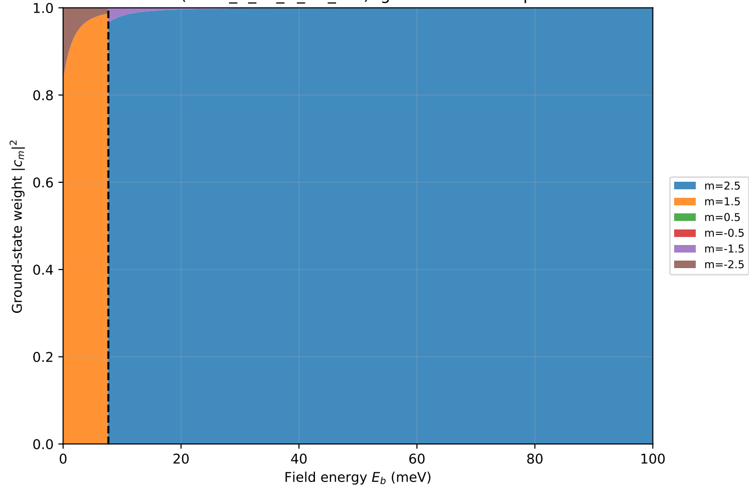
CeIn3 (cubic_B_Td_O_Oh_like): ground-state composition
