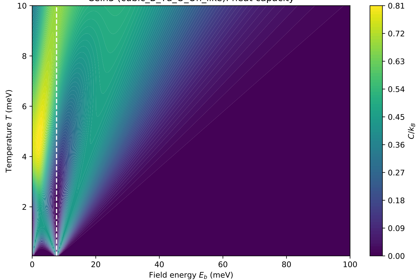
CeIn3 (cubic_B_Td_O_Oh_like): heat capacity
