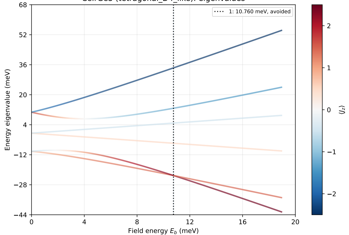
CeIrGe3 (tetragonal_D4_like): eigenvalues
