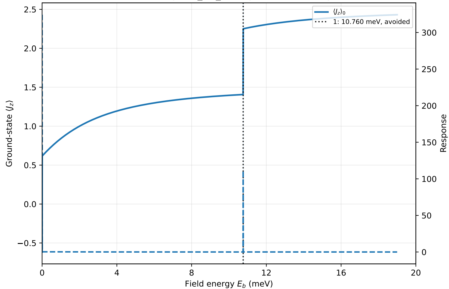
CeIrGe3 (tetragonal_D4_like): ground-state response
