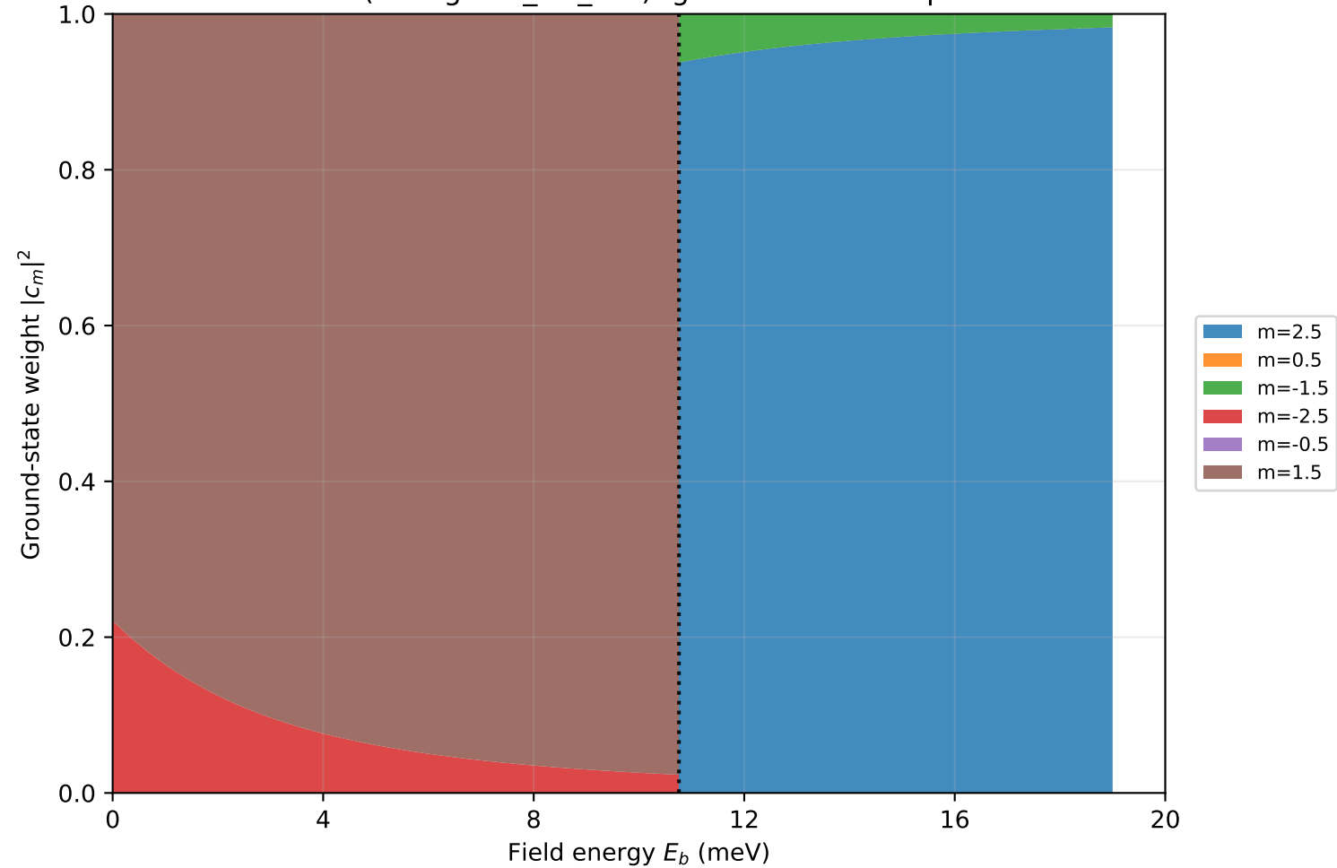
CeIrGe3 (tetragonal_D4_like): ground-state composition
