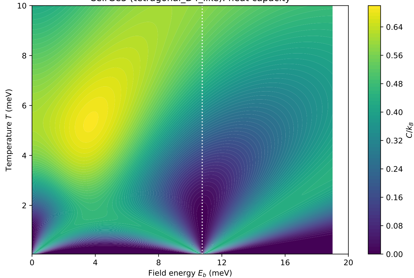
CelrGe3 (tetragonal_D4_like): heat capacity
