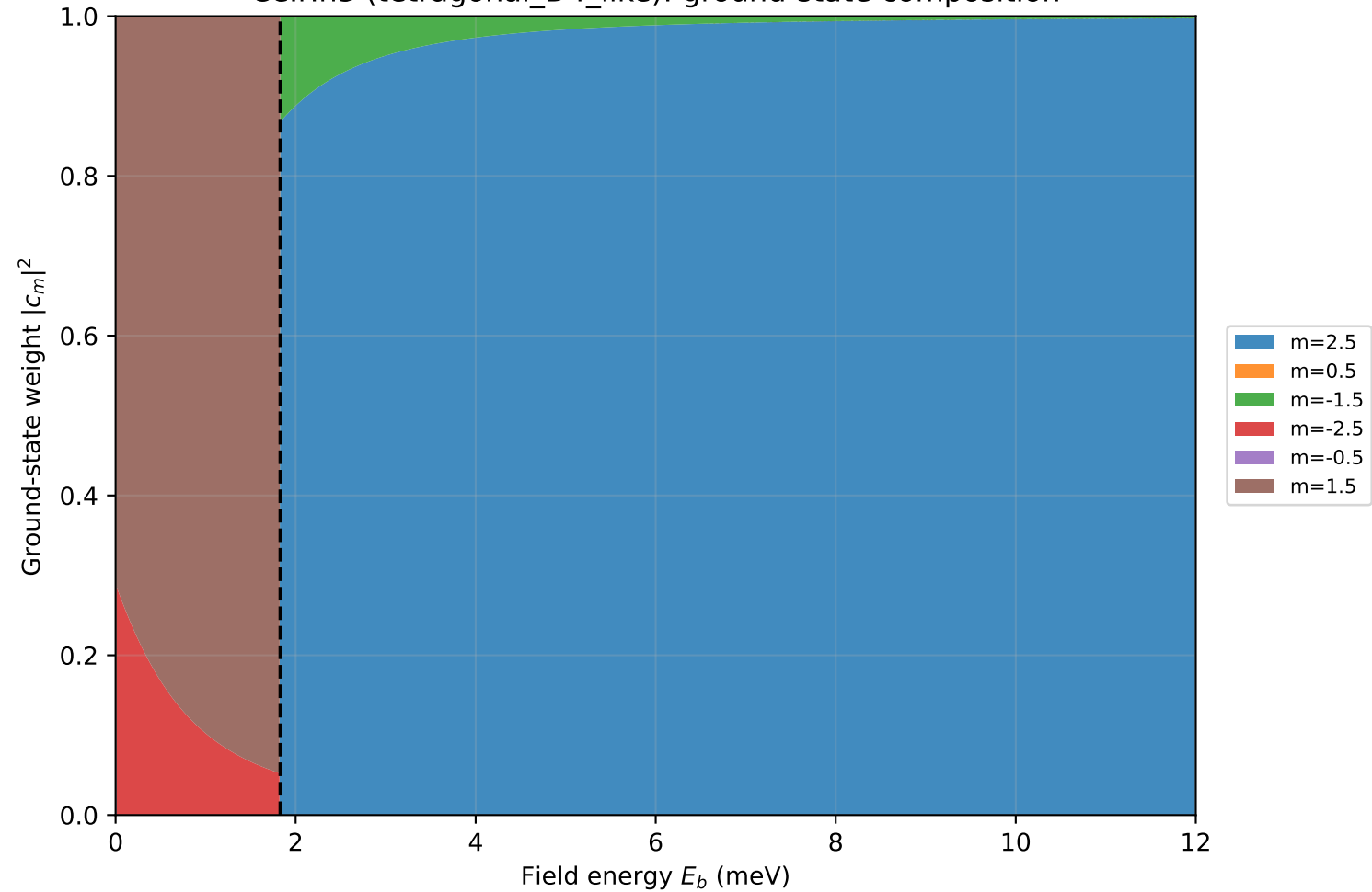
CeIrIn5 (tetragonal_D4_like): ground-state composition
