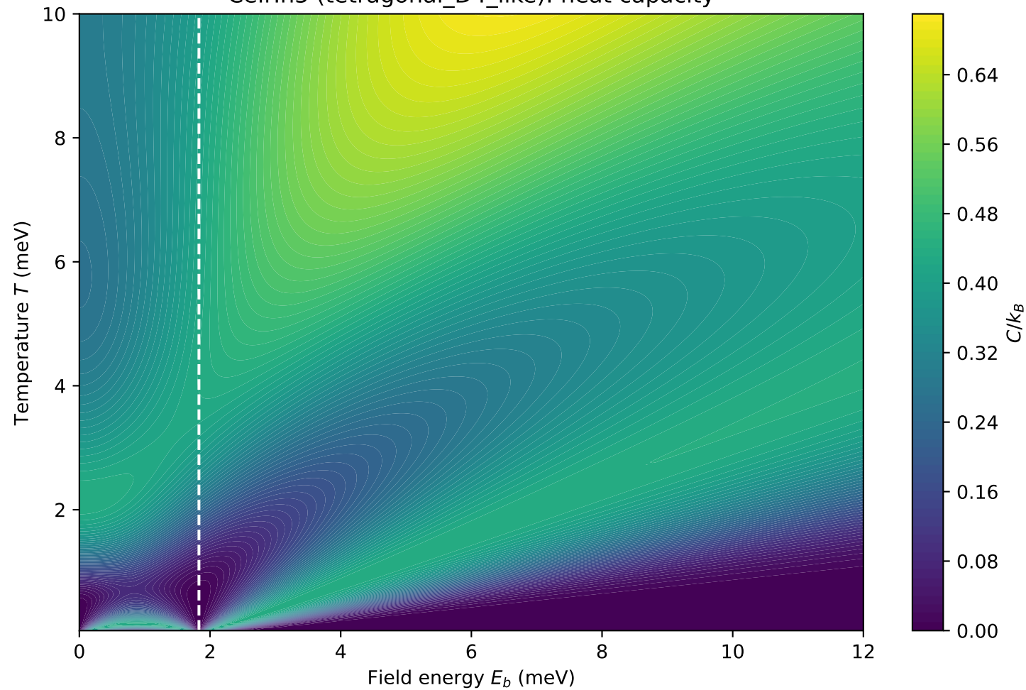
CeIrIn5 (tetragonal_D4_like): heat capacity
