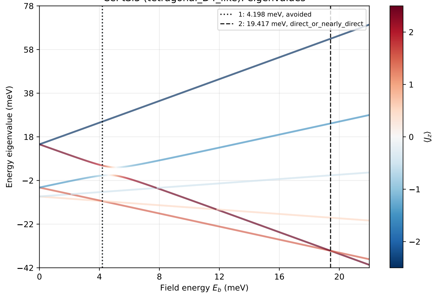
CePtSi3 (tetragonal_D4_like): eigenvalues
