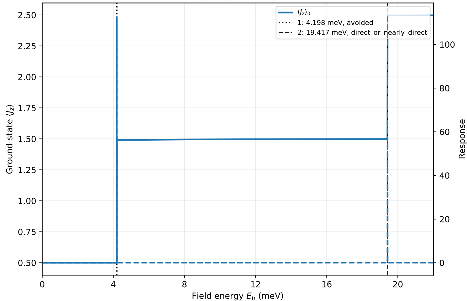
CePtSi3 (tetragonal_D4_like): ground-state response
