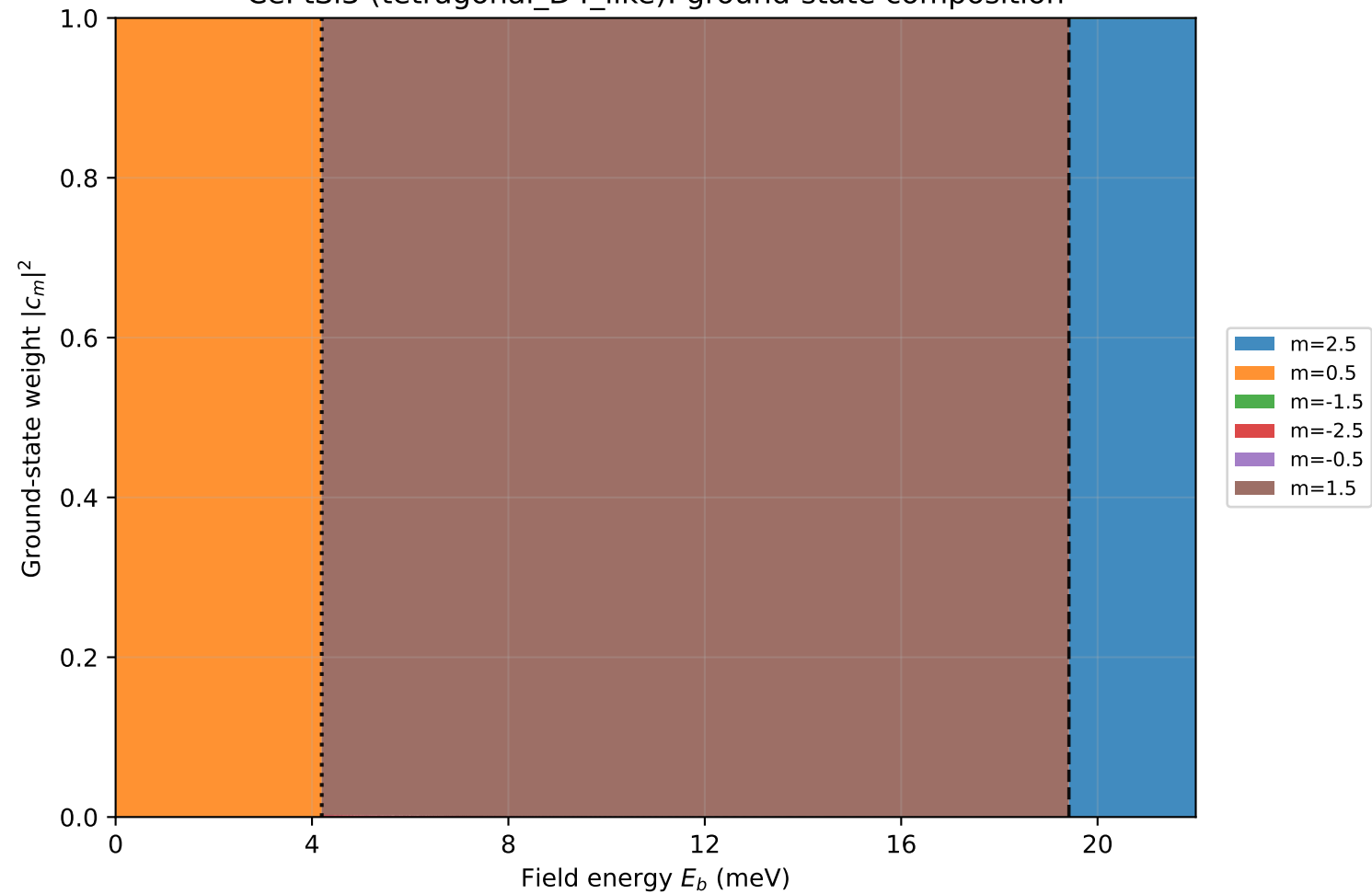
CePtSi3 (tetragonal_D4_like): ground-state composition
