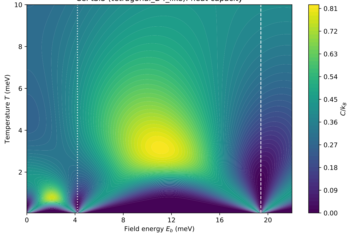
CePtSi3 (tetragonal_D4_like): heat capacity
