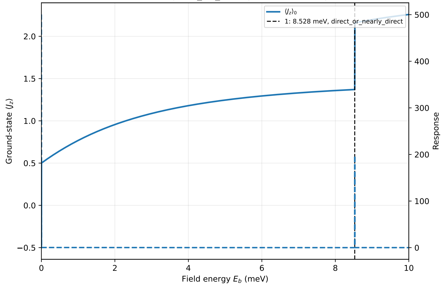
CeRhGe3 (tetragonal_D4_like): ground-state response
