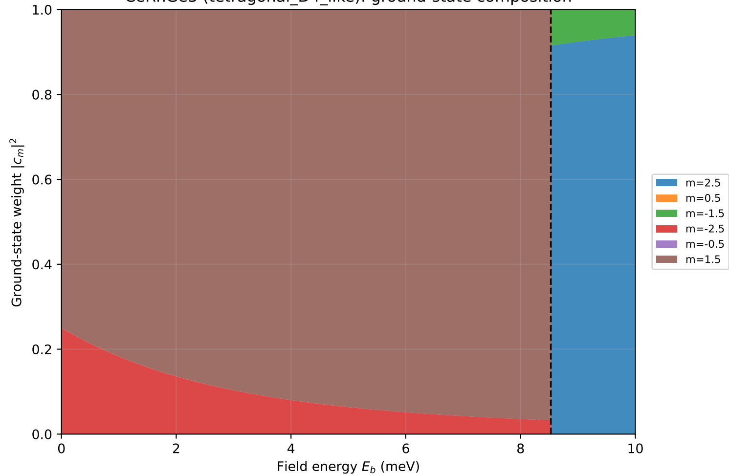
CeRhGe3 (tetragonal_D4_like): ground-state composition
