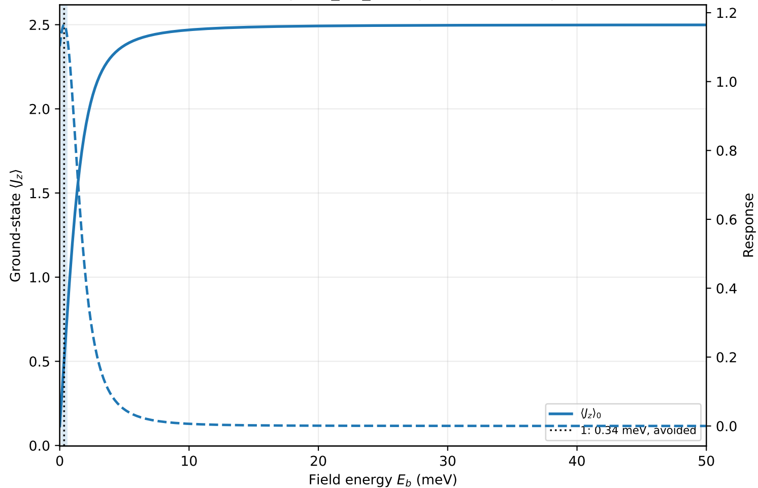
CeRhIn5 (tetragonal_D4_like): ground-state response
