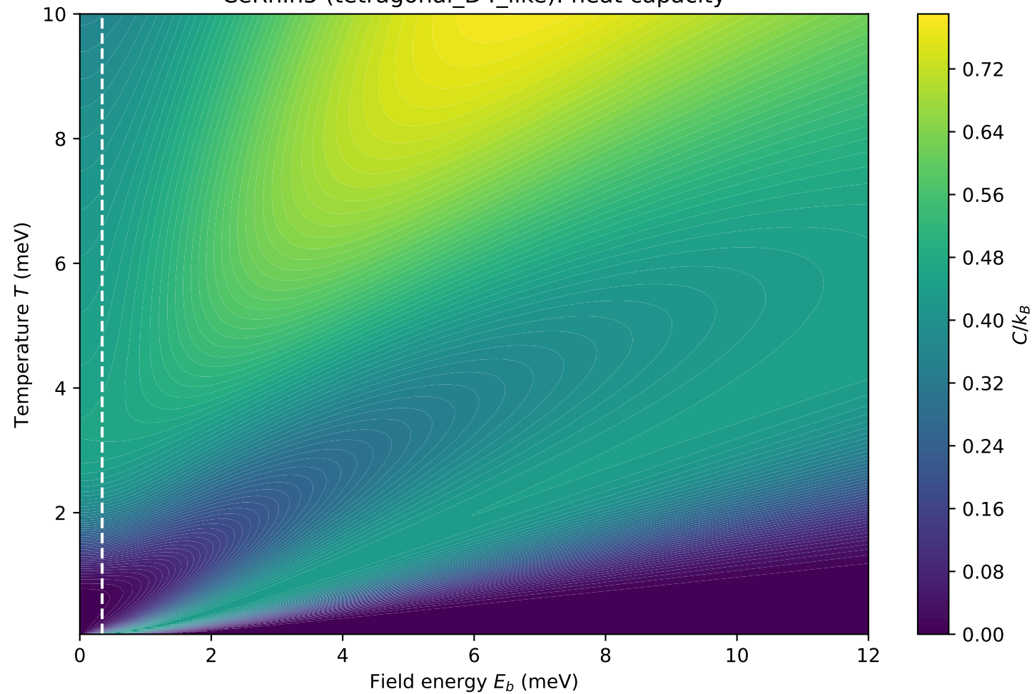
CeRhIn5 (tetragonal_D4_like): heat capacity
