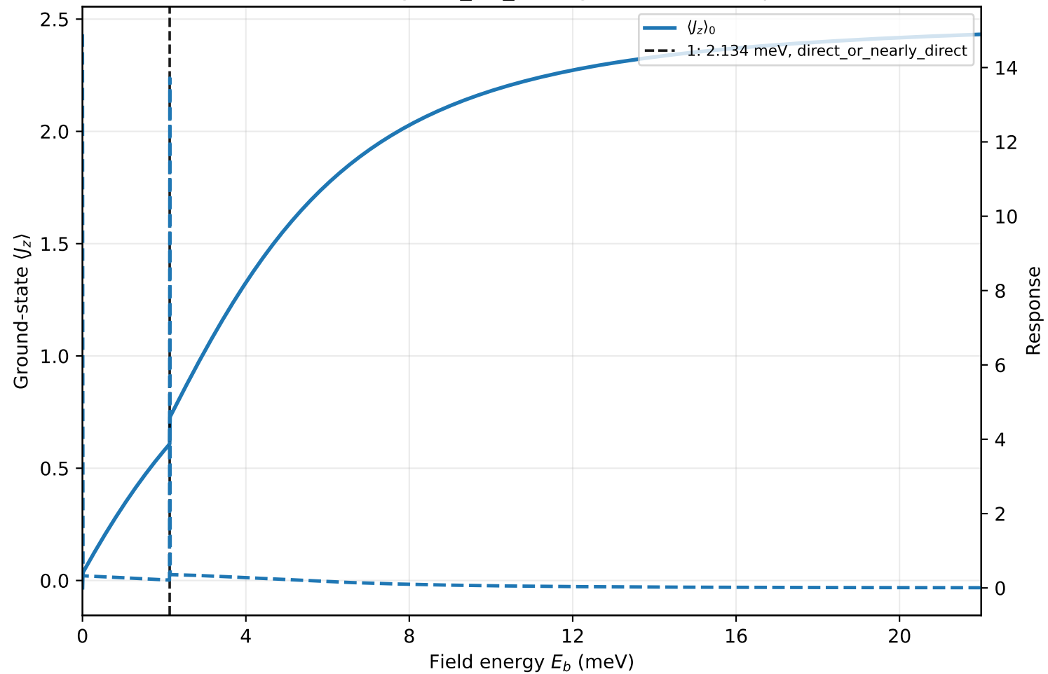
CeRhSi3 (tetragonal_D4_like): ground-state response
