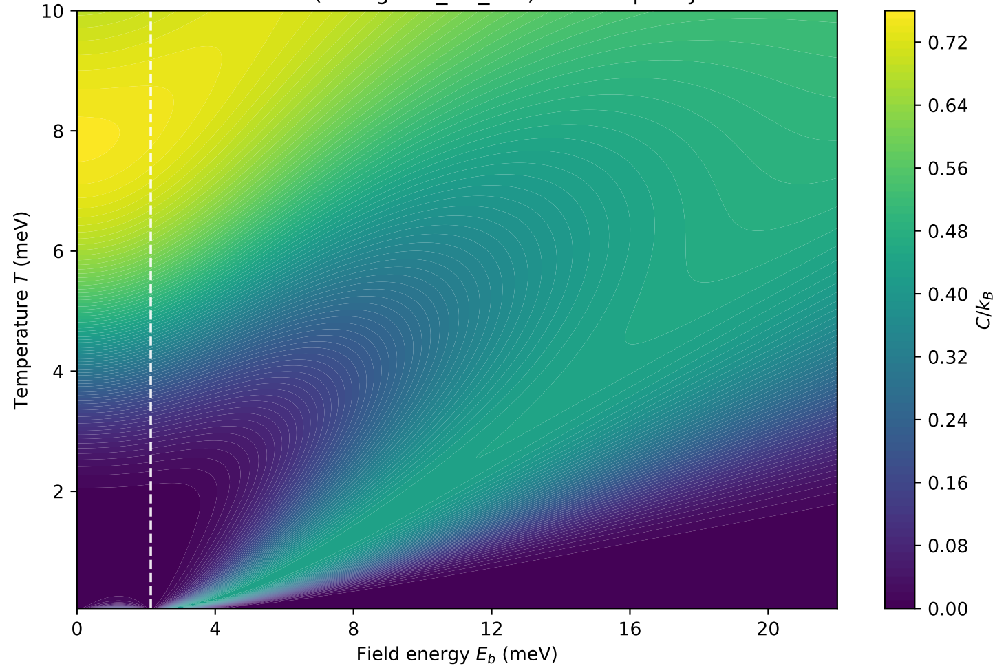
CeRhSi3 (tetragonal_D4_like): heat capacity
