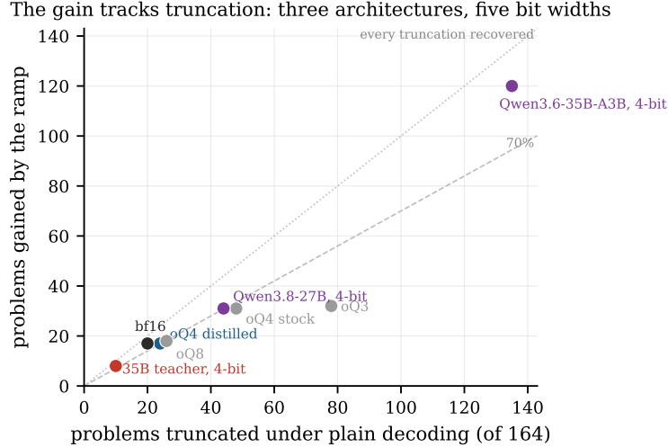
Figure 4: Ramp gain against plain-decoding truncation count, one point per build, HumanEval at 2,048 (Table 8). The dotted line is every truncation recovered; the dashed line is 70%. Full precision, the dense Qwen and the MoE Qwen sit on the same line as the quantized Ornith builds.
