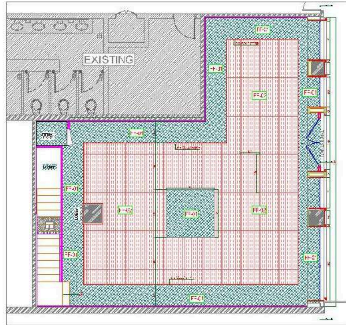
GROUND FLOOR FLOOR FINISHES LAYOUT
