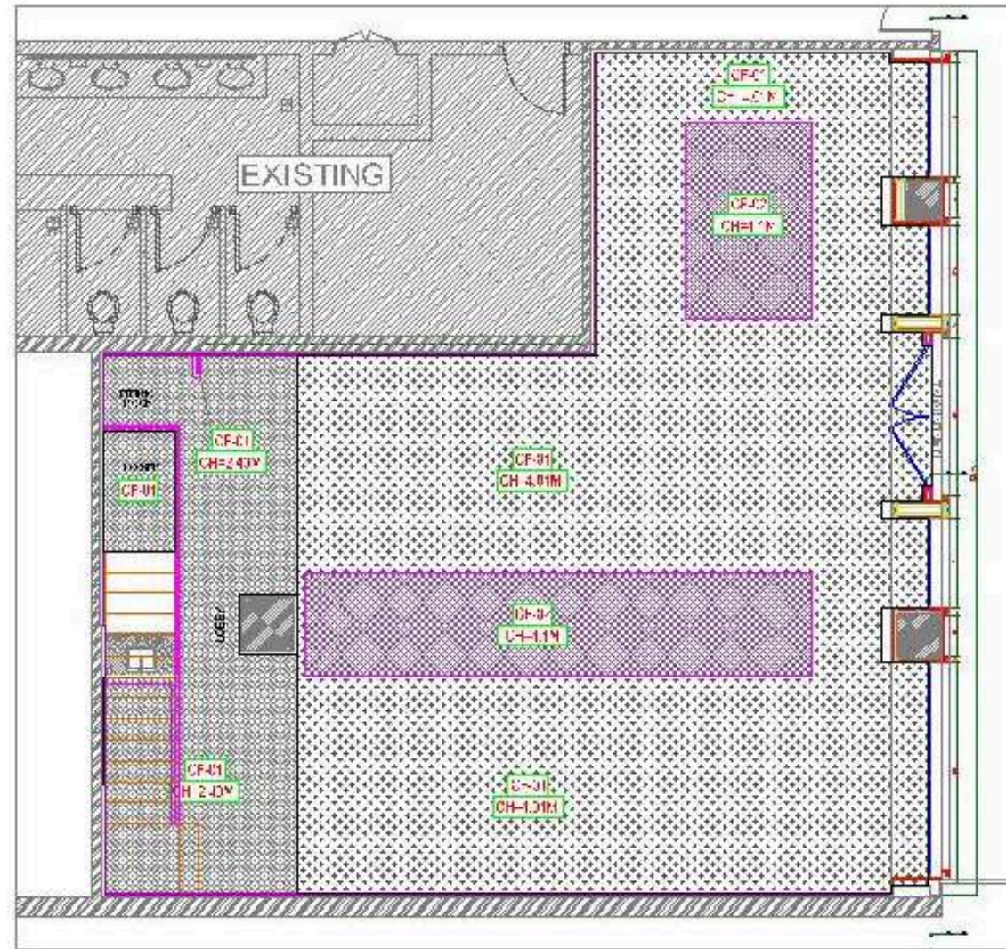
GROUND FLOOR CEILING FINISHES LAYOUT
