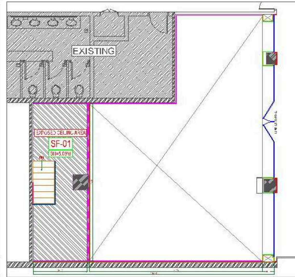
MEZZANINE FLOOR CEILING FINISHES LAYOUT
