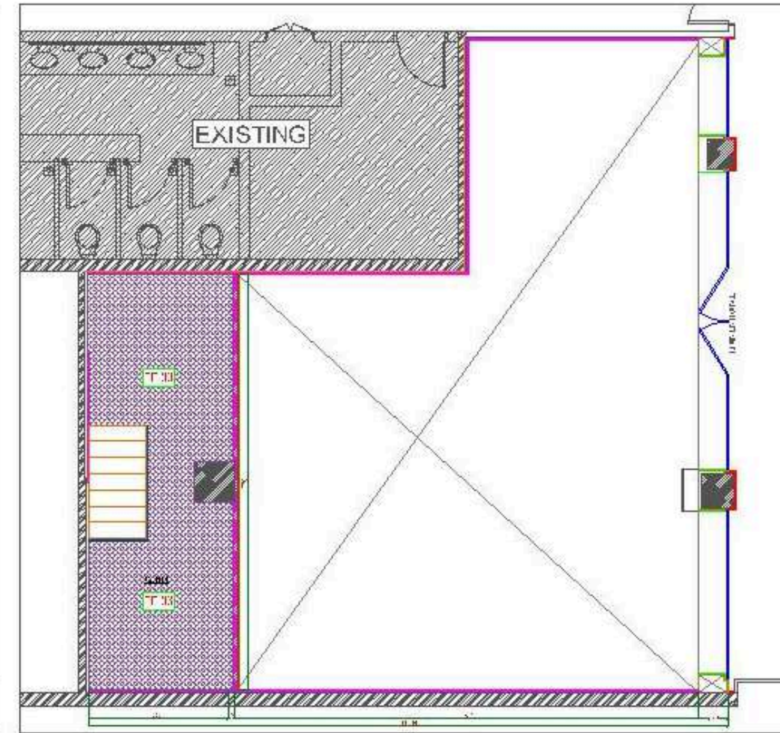
MEZZANINE FLOOR FLOOR FINISHES LAYOUT
