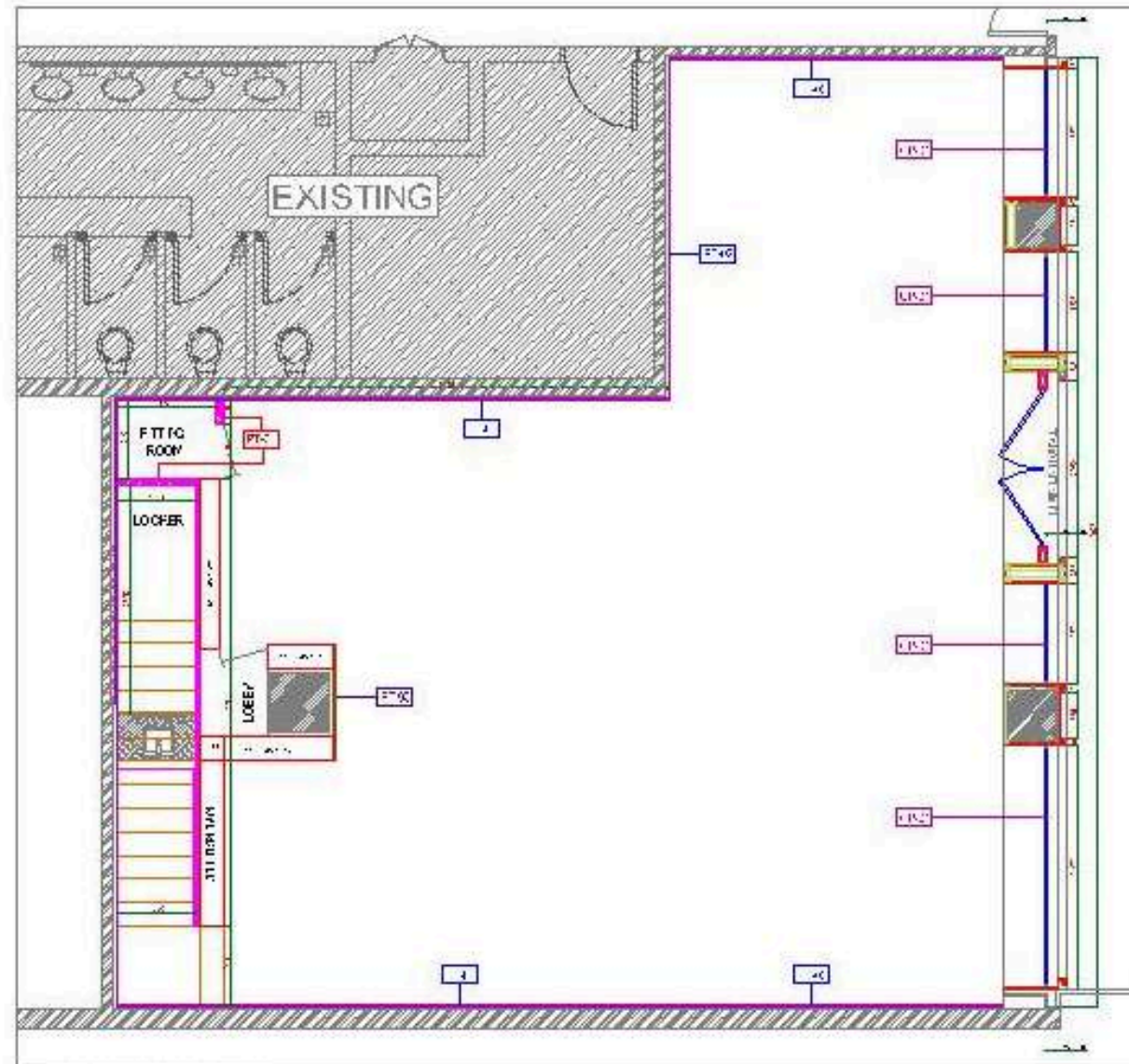
GROUND FLOOR PARTITION LAYOUT
