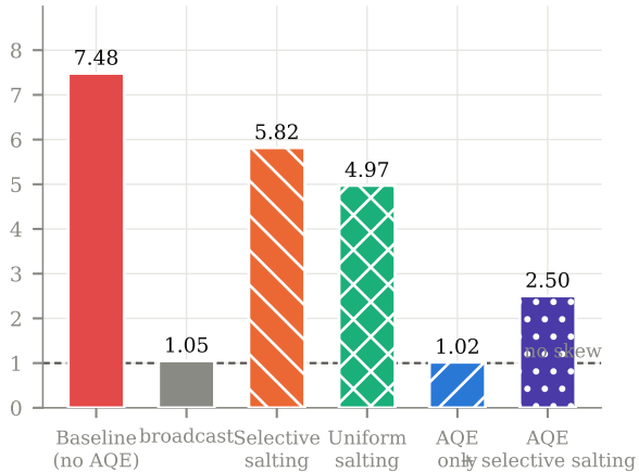
Residual skew by strategy ( P = 10 )
