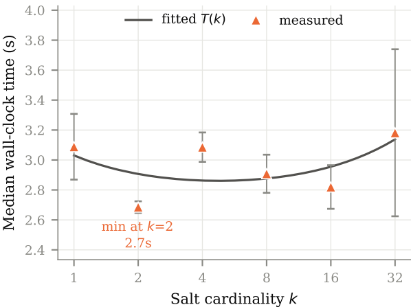
Salt cardinality vs. runtime, P = 11
