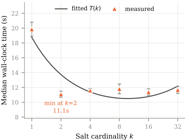
Salt cardinality vs. runtime, P = 321
