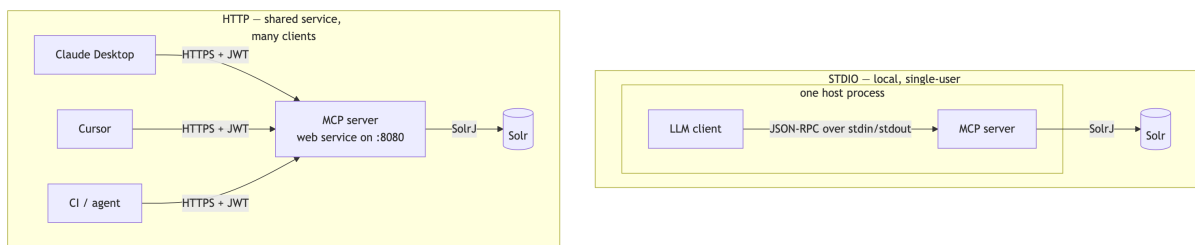
Figure 6: The two transports as topologies: in STUDIO the client spawns the server as a child process and they share one process over stdin/stdout (one user); in HTTP one long-lived server fronts many clients over authenticated HTTPS.
