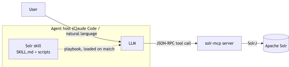
Figure 2: Skills and MCP are different layers of the agent stack: a skill is the playbook loaded into the model (what to do), while MCP is the hands that execute it against a live system (how to act). Here a Solr skill drives the solr-mcp search tool.
