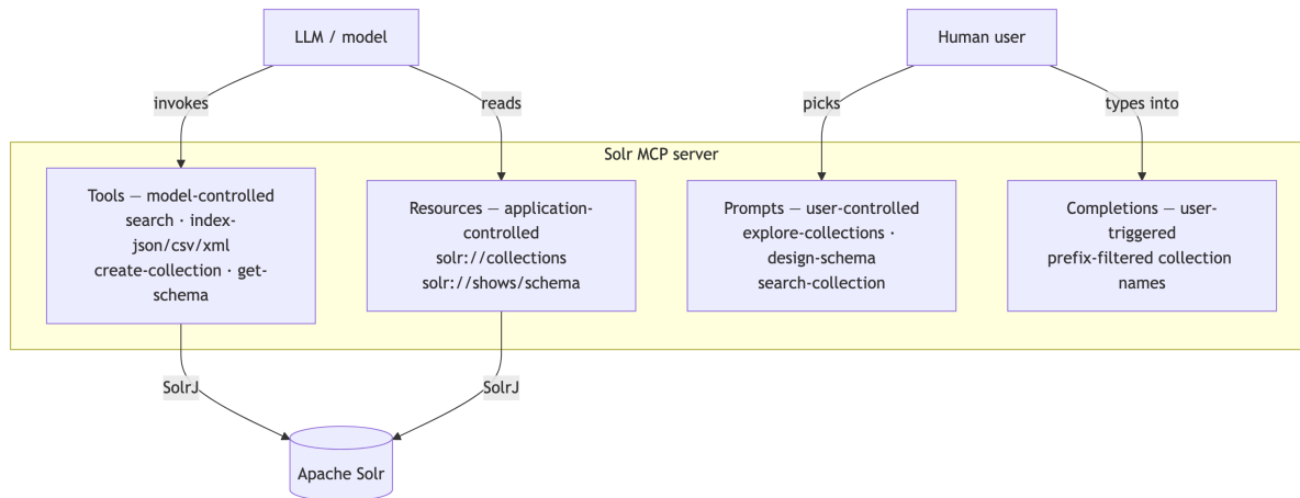
Figure 4: The four primitives by who controls them: the model invokes tools and reads resources; the user picks prompts and types into completions. Only tools and resources reach Solr — prompts and completions stay in the client.
