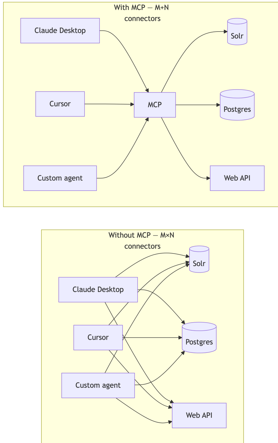
Figure 1: The M \times N integration problem and MCP's M+N answer: without a shared protocol every client needs a bespoke connector to every system; with MCP each client and each system implements one protocol once.
