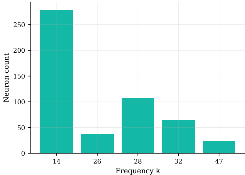
MLP neurons per frequency
