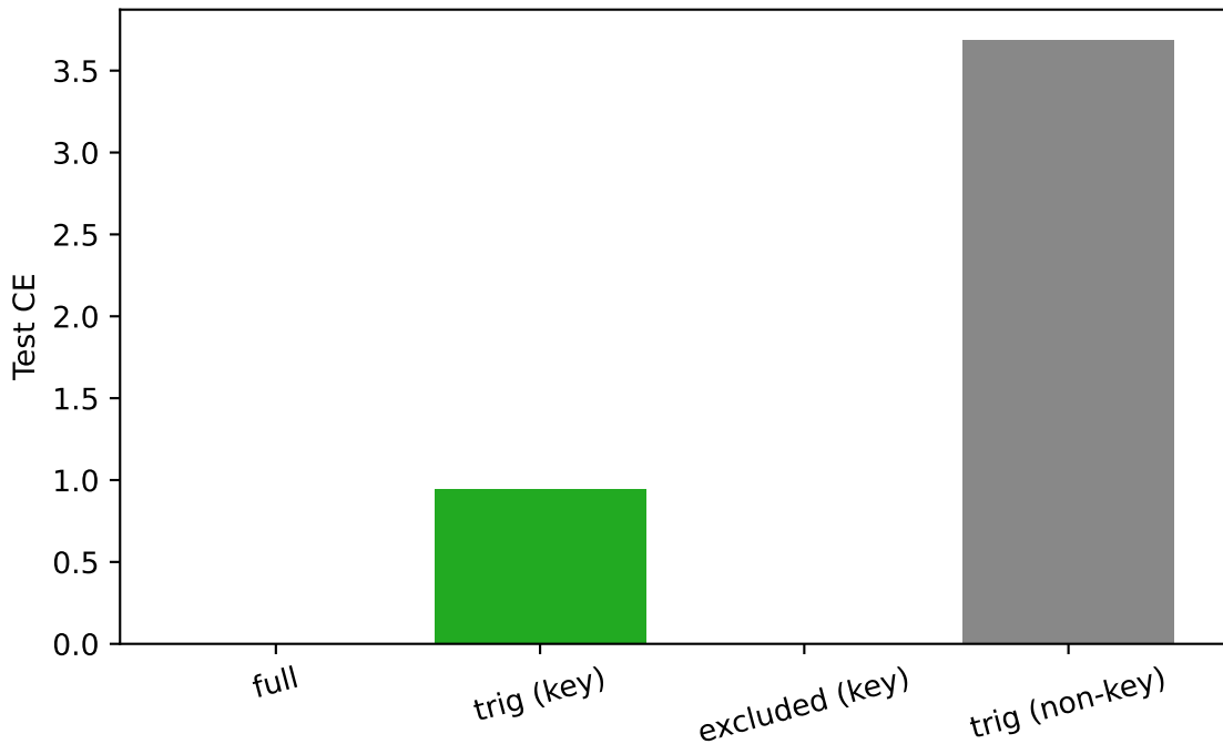
Frequency ablations (Nanda §4.4)
