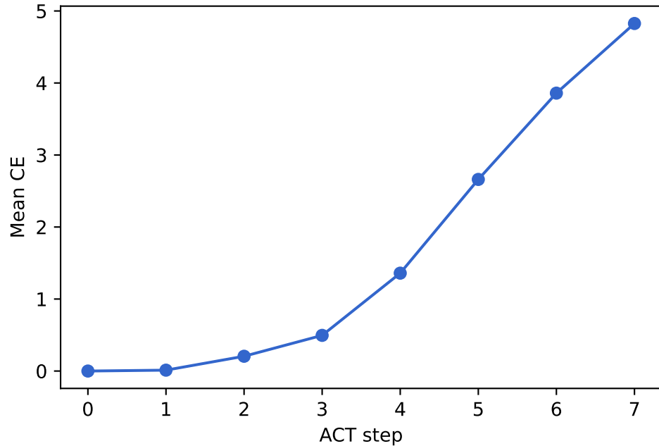
Mean-field loss along recursion (HRM §4.1)
