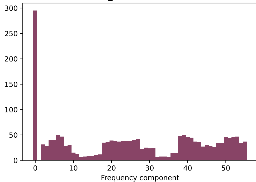
Excluded loss per frequency
