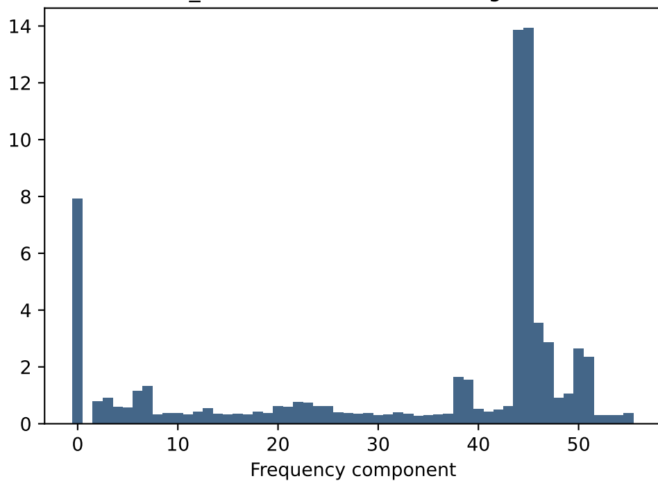
Progress measures at final ckpt (Nanda §5)
