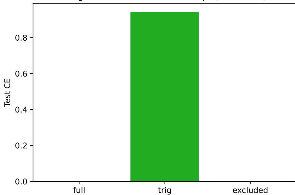
Progress measures at final ckpt (Nanda §5)
