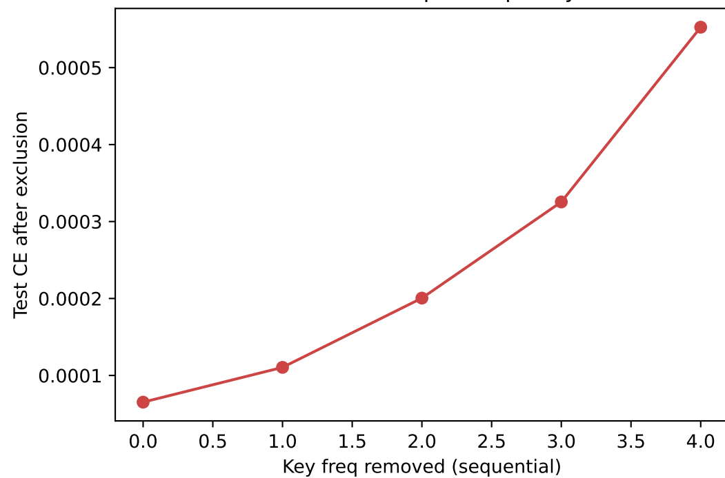
Excluded loss per frequency
