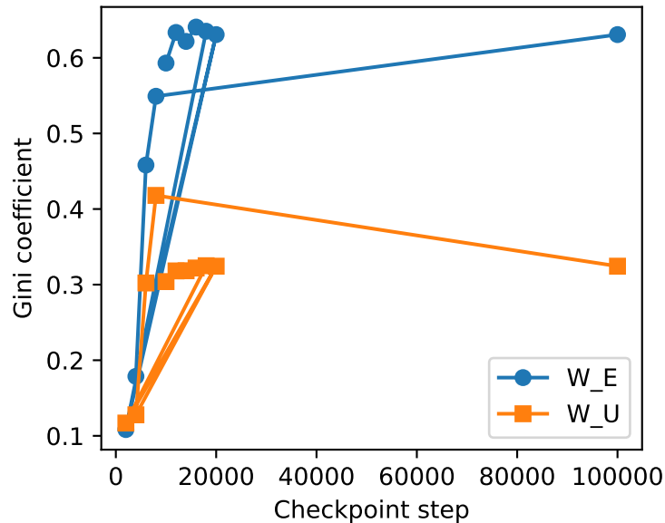
Fourier sparsity dynamics
