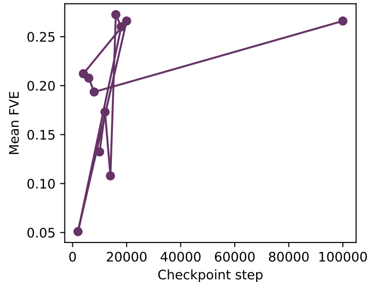
Trig logit FVE over training
