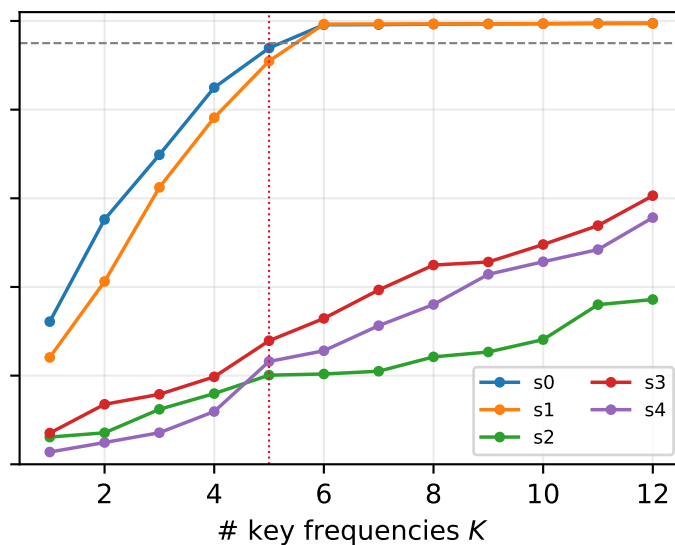
TRM minimal
