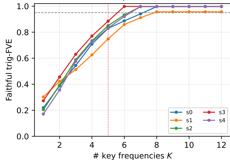
Nanda 1-layer (calibration)
