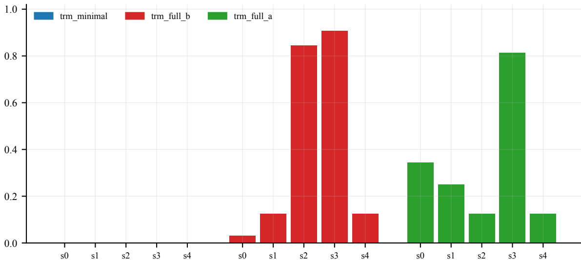
Fixed-point violation rate
