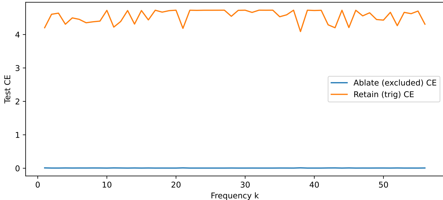
All-frequency ablations (trm_full_a)
