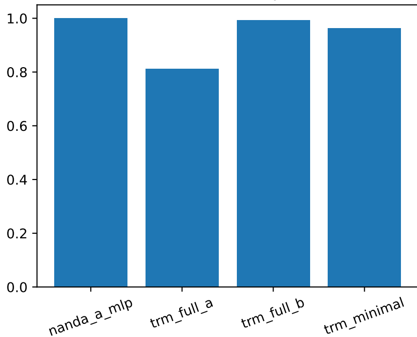
Test accuracy
