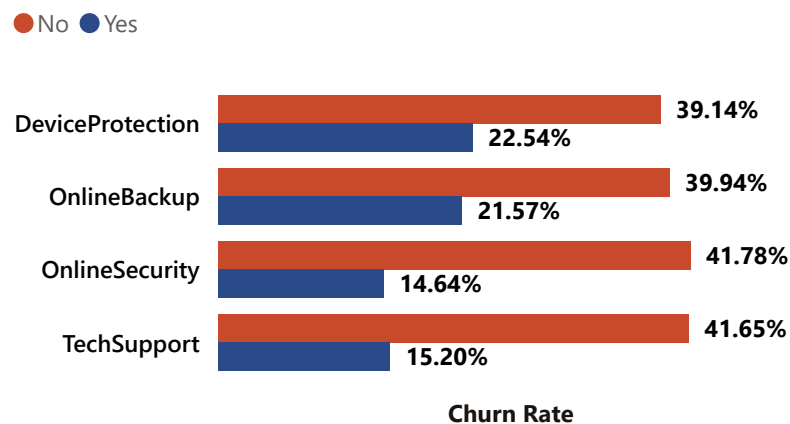
Churn Rate by Add-on Services
