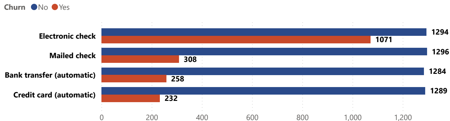
Churn By Payment Method
