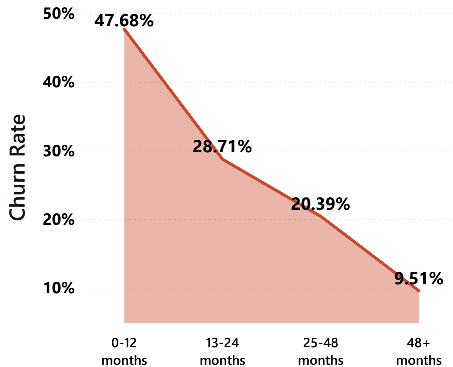
Churn Rate by Tenure
