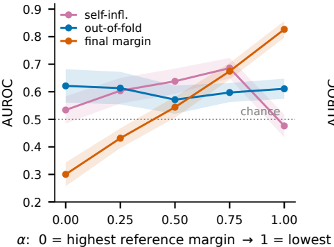
(a) margin-targeted sweep
