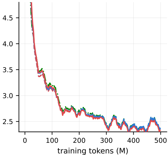
training loss (nats)
