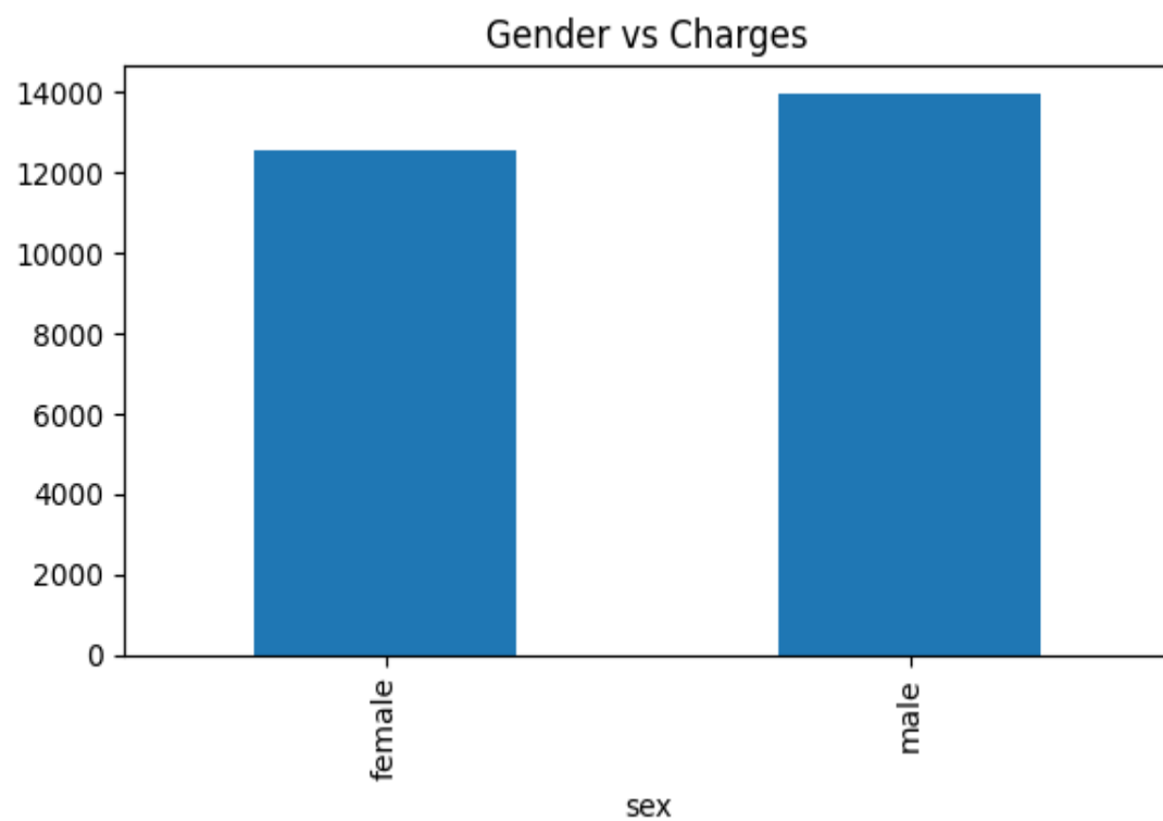
Gender vs Charges
