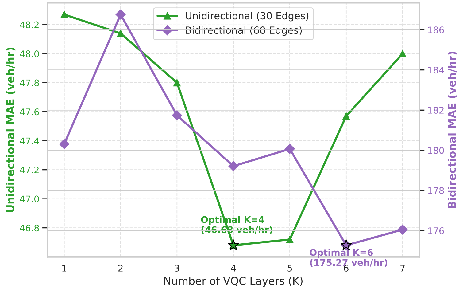
Hierarchical Network Forecasting (24 Nodes): MAE vs. VQC Layers (K)
