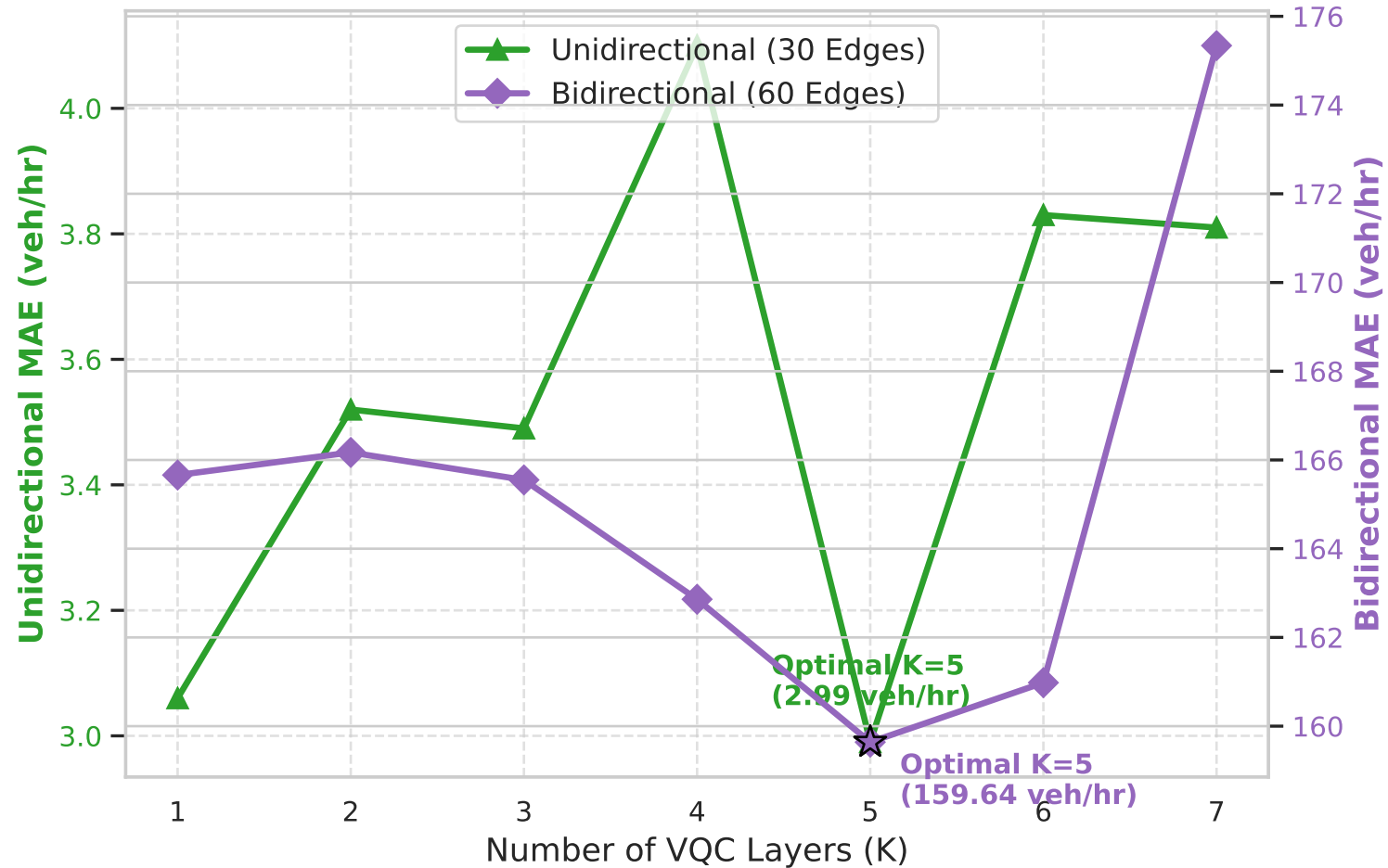
Hierarchical Network (24 Nodes, 3 Zones): MAE vs. VQC Layers (K)
