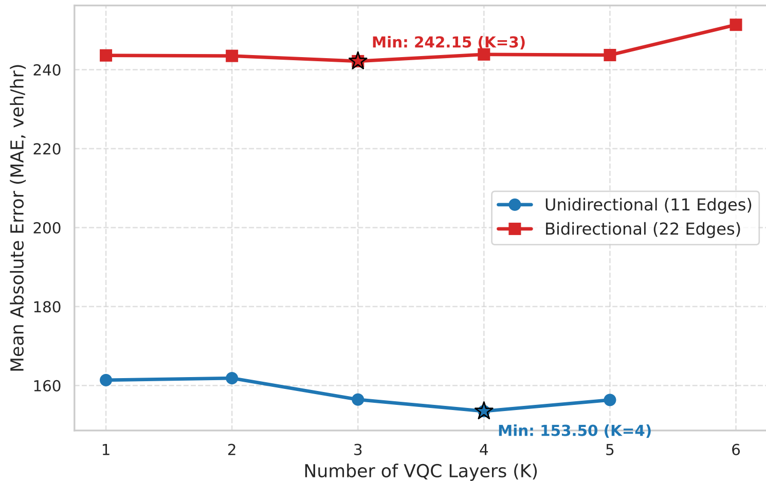
Single Network (8 Nodes): MAE vs. VQC Layers (K)
