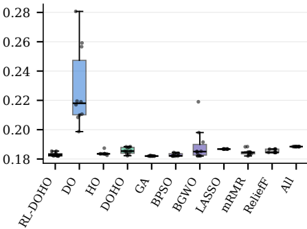
Final fitness (lower is better)
