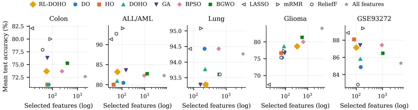
Fig. 8. Mean test accuracy against mean number of selected features (log scale) on the gene-expression datasets. Hollow markers are filter or embedded methods.
