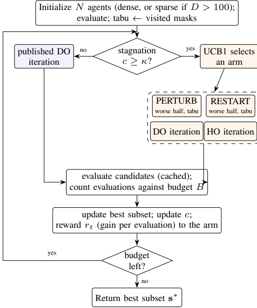
Fig. 2. Flow of one RL-DOHO run. Published DO iterations are used while the best subset improves; after \kappa = 2 iterations without an accepted change, the UCB1 controller chooses one of four arms for the next step. The run stops when the evaluation budget is spent.
