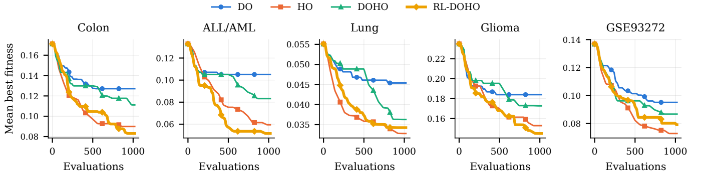
Fig. 7. Mean best fitness against fitness evaluations, over ten seeds, on the gene-expression datasets for the DO–HO family (20 agents, 1,020 evaluations).
