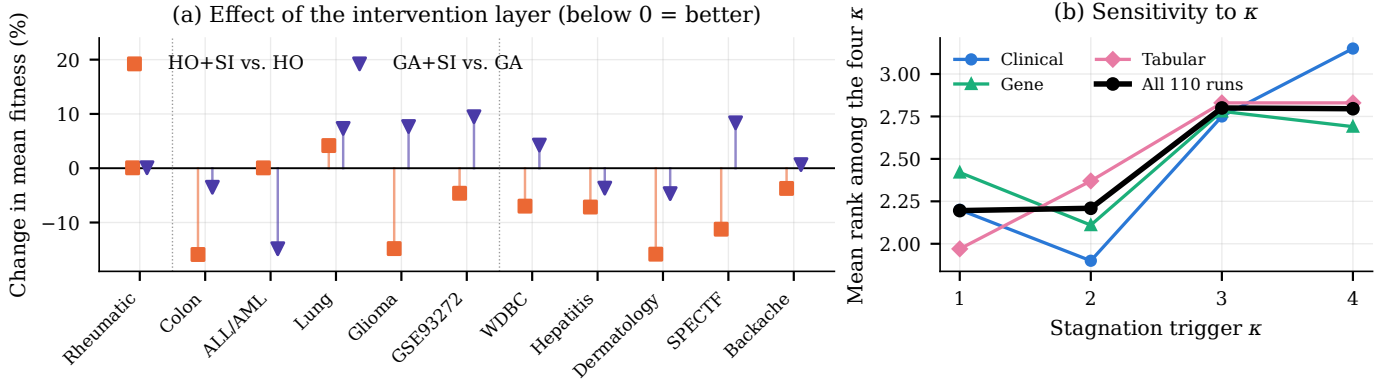
Fig. 12. (a) Change in mean fitness when the intervention layer is added to HO and to the GA, per dataset (negative is better); dotted lines separate the clinical, gene-expression and tabular datasets. (b) Mean per-run rank of RL-DOHO’s fitness among the four values of the stagnation trigger \kappa , by data type and over all 110 runs.
