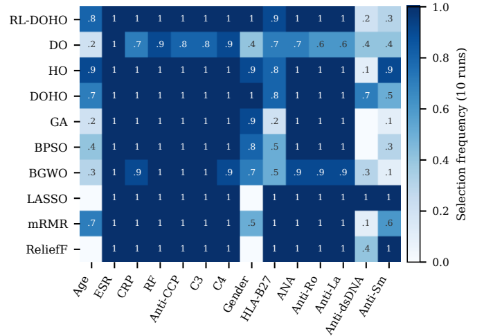
Fig. 6. Rheumatic data: fraction of the ten runs in which each method selected each variable (blank = never).
