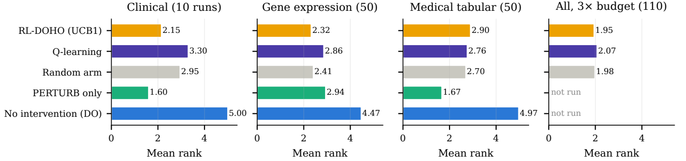
Fig. 10. Mean per-run fitness rank of the controller variants within each group of runs (lower is better). “No intervention” is the published DO; it was not run at three times the budget.
