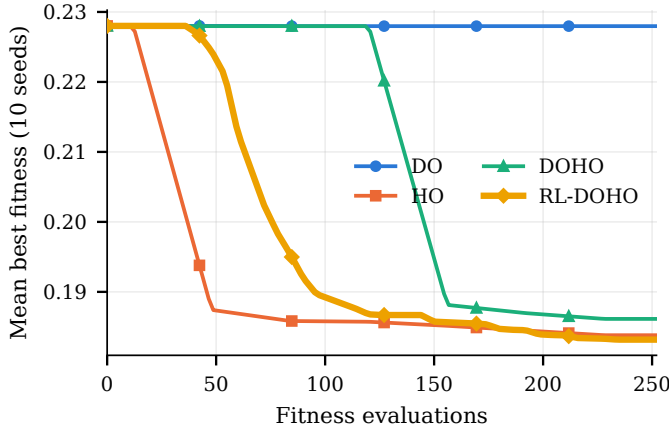
Fig. 5. Mean best fitness against fitness evaluations used, over ten seeds, on the rheumatic data for the DO-HO family.
