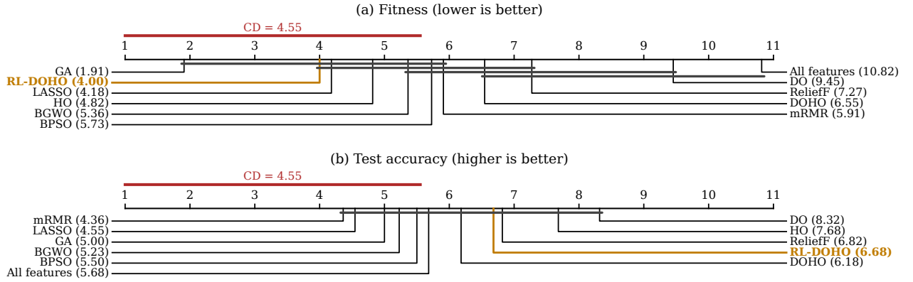
Fig. 9. Critical-difference diagrams over the eleven datasets (methods ranked by their mean on each dataset; Nemenyi test, \alpha = 0.05 , CD = 4.55 ). Thick bars join methods whose average ranks differ by less than the critical difference. Labels are split between the two sides for readability: a method's rank is given by where its line meets the axis (further left is better), not by its label's side or vertical position.
