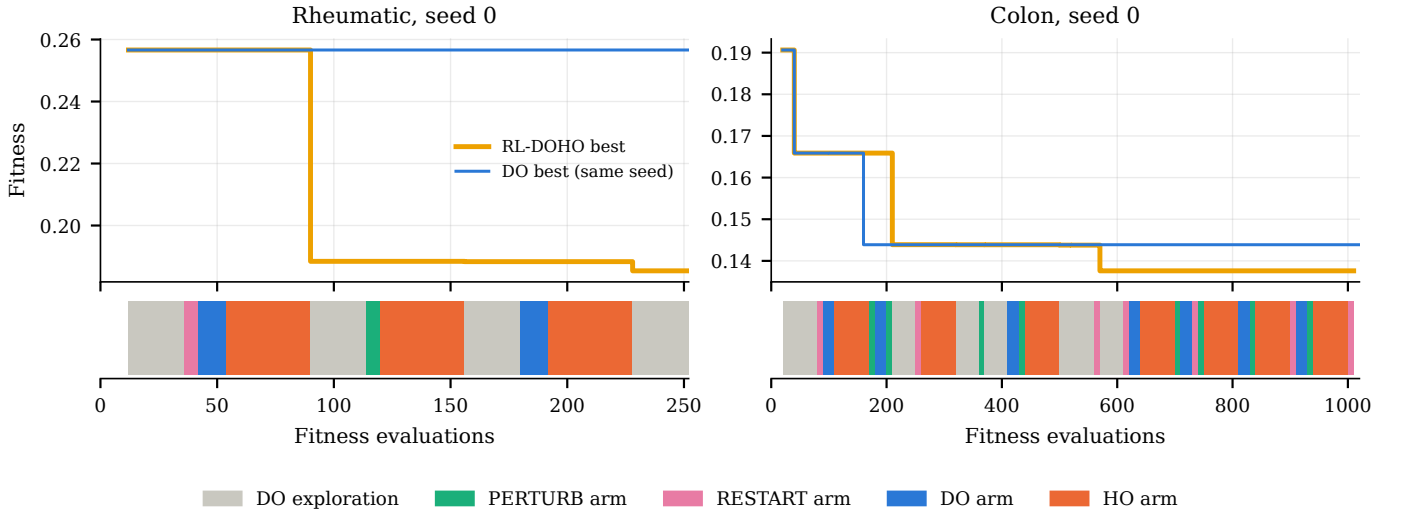
Fig. 11. Best fitness of RL-DOHO and DO for seed 0 on the rheumatic data and on Colon, against evaluations used, with RL-DOHO’s action at each step (bottom). On the rheumatic data DO never improves on its initial best with this seed.
