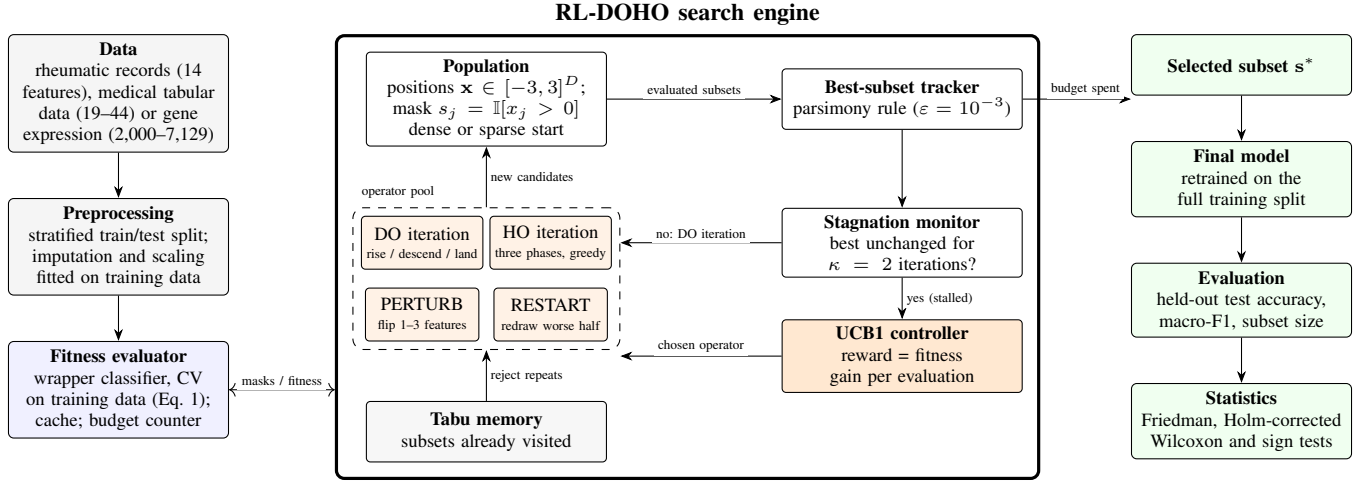
Fig. 1. Architecture of the feature-selection pipeline. The data are split and preprocessed, and every candidate subset is scored by the wrapper fitness on the training data only, with a cache and a counter that enforces the evaluation budget. Inside the RL-DOHO engine, the population is updated by published DO iterations while the best subset improves. When the stagnation monitor detects \kappa = 2 stalled iterations, the UCB1 controller chooses one operator from the pool, rewarded by the fitness gain per evaluation, and tabu memory rejects subsets already visited. When the budget is spent, the selected subset is used to retrain the final classifier, which is evaluated on held-out data.
