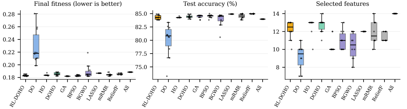
Fig. 4. Rheumatic data: distribution over ten seeds of final fitness, test accuracy and subset size for every method (dots are individual runs; “All” is the full feature set).
