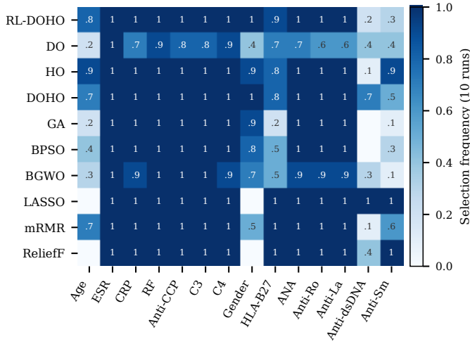
Fig. 6. Rheumatic data: fraction of the ten runs in which each method selected each variable (blank = never).
