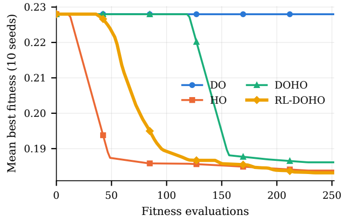
Fig. 5. Mean best fitness against fitness evaluations used, over ten seeds, on the rheumatic data for the DO–HO family.
