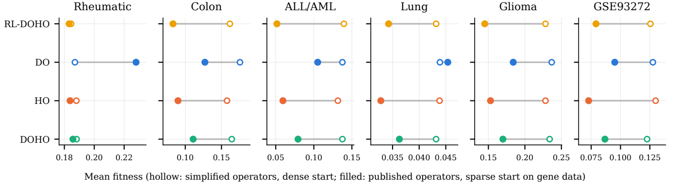
Fig. S1. Mean fitness of the DO–HO family under the earlier configuration (hollow) and the final one (filled), per dataset.
